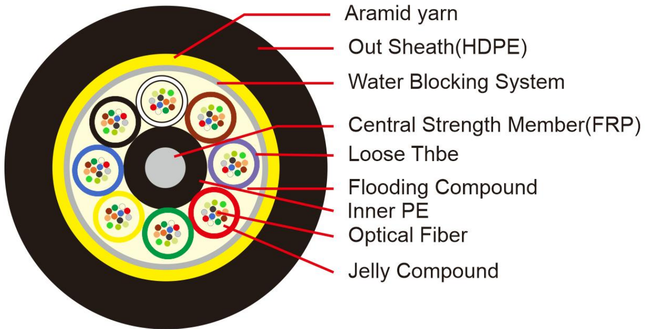
ADSS-SS-200m-144cores Schematic for reference only
